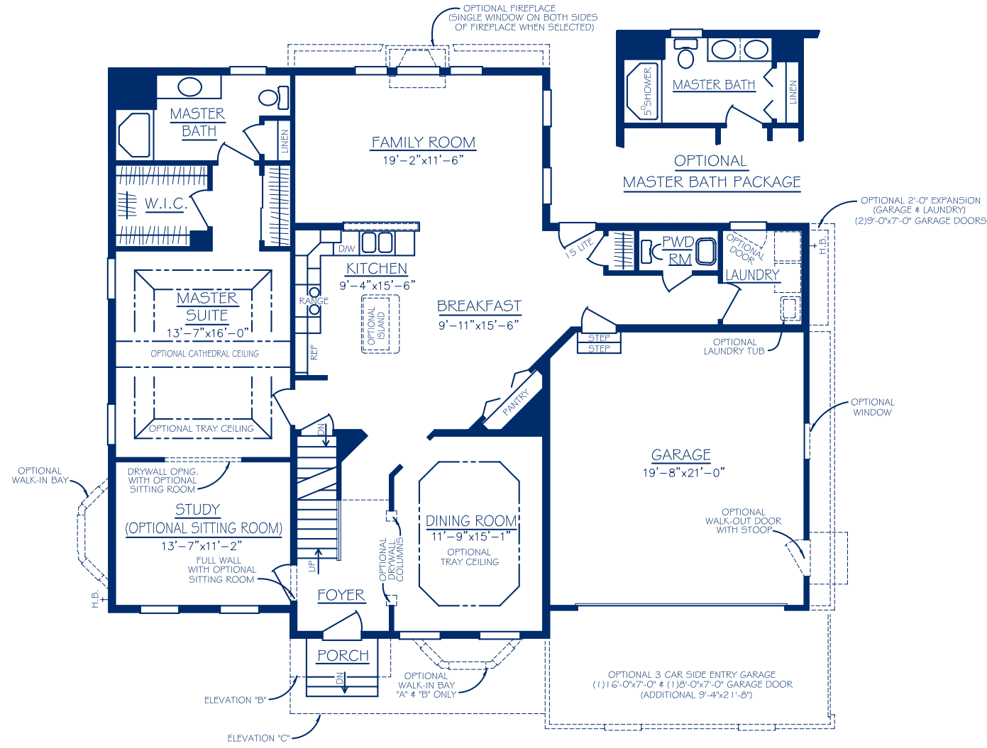
FIRST FLOOR
