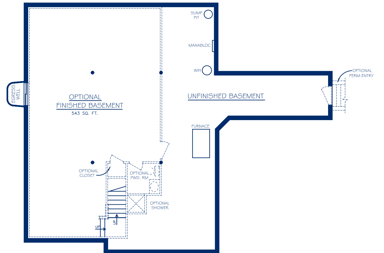
FOUNDATION
