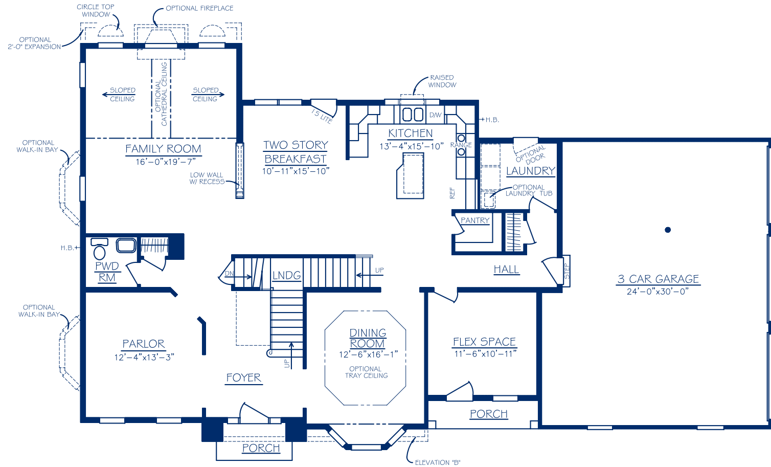
FIRST FLOOR
