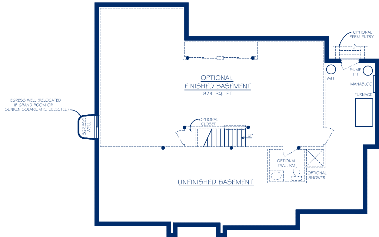
FOUNDATION
