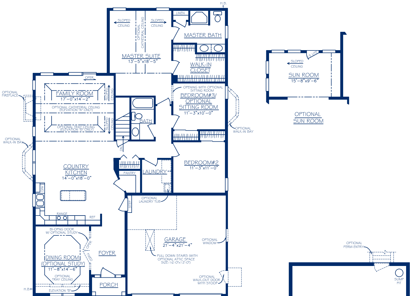
FIRST FLOOR WITH OPTIONAL FOUNDATION
