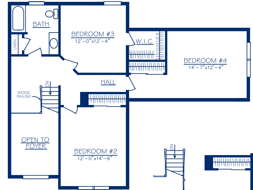
OPTIONAL SECOND FLOOR WITH 4th BEDROOM *B* - 3092 SQ. FT. *C* - 3092 SQ. FT.
