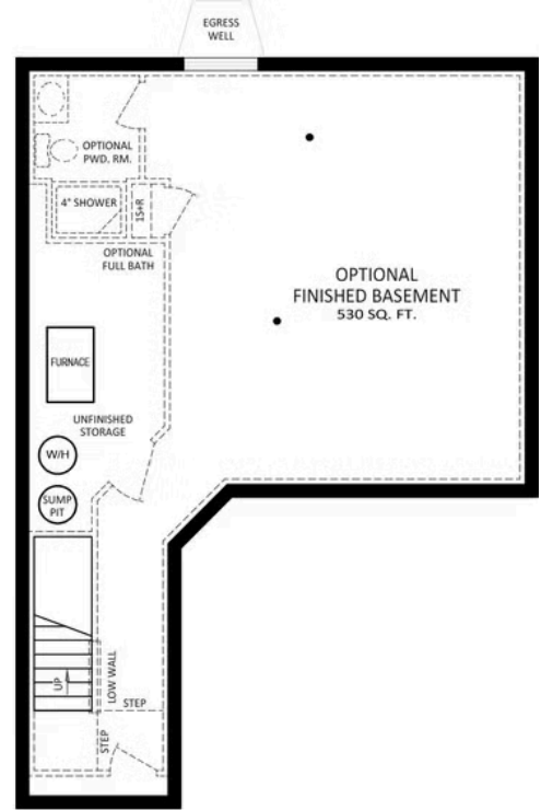
OPTIONAL FIRST FLOOR EXPANSION FOUNDATION PLAN
