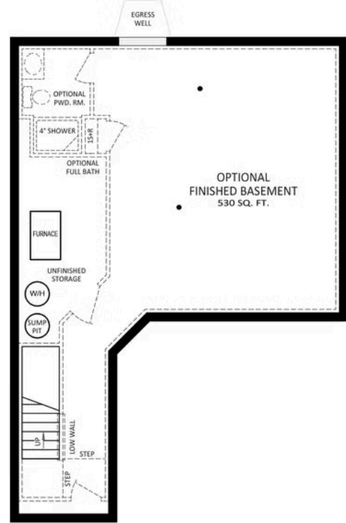
OPTIONAL FIRST FLOOR EXPANSION FOUNDATION PLAN
