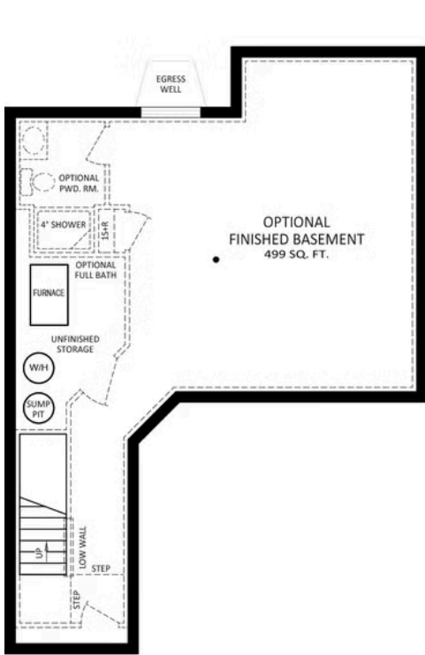
OPTIONAL BREAKFAST EXPANSION FOUNDATION PLAN
