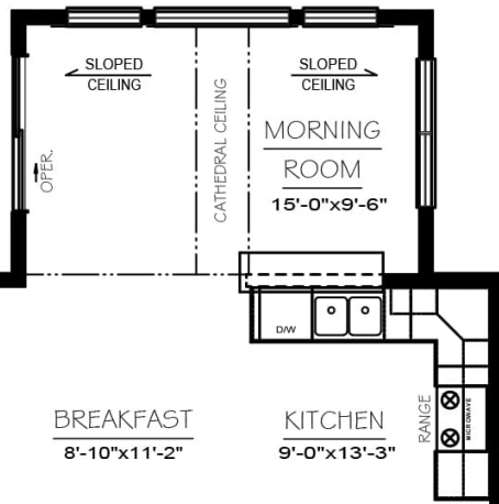
OPTIONAL MORNING ROOM
